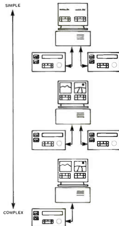
Figure 2. Different approaches to off-line system construction. The simplest systems use a computer to operate VTRs. More complex systems drive VTRs with a computer, but show a representation of the video on the computer screen. The most sophisticated and powerful systems digitize and process the video, or a compressed representation of it, in the computer itself.
