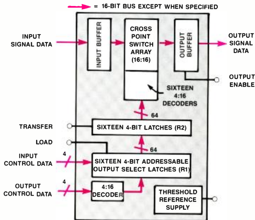
Figure 1. This 16×16 digital crosspoint switch features a double row of input/output select latches (center). While the switch is active (transmitting) prior to a reconfiguration, the first row of input/output select latches (R1) is serially loaded at a rate of 3ns per I/O selection. When all I/Os to be changed have been loaded in R1, the content of R1 is parallel-transferred to the second row of select latches (R2), resulting in a complete switch reconfiguration in just 3.6ns. No data dropout occurs for any output whose input connection does not change.
