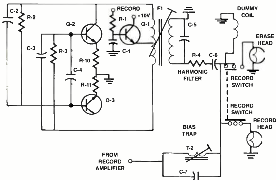
Figure 1. Diagram of a typical bias oscillator circuit.
